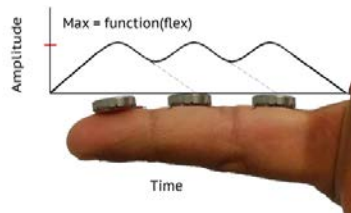
Figure 3: Vibrotactile Waveform
